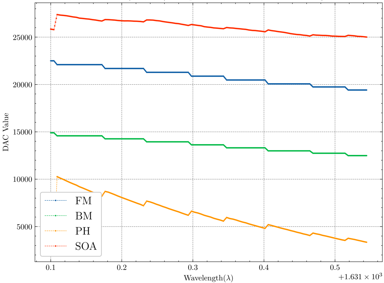
DAC Parameters (800, 900) Interpolated with 3 Intermediate Integer Values
